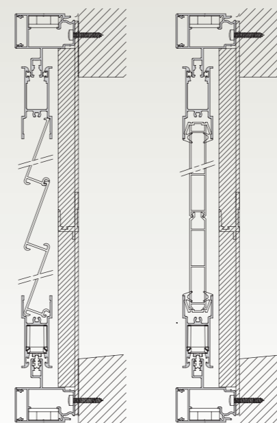
VOLETS COULISSANTS
